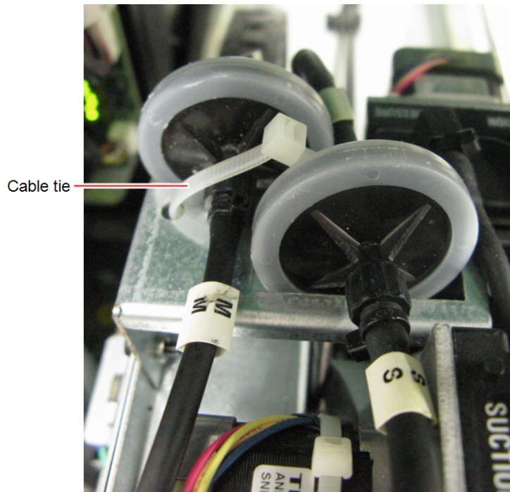
Figure 6-110 Material filters secured to the printer
