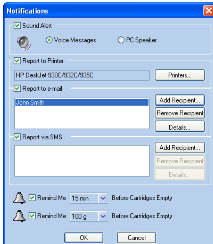
Figure 5-96 Notifications dialog box (server)
