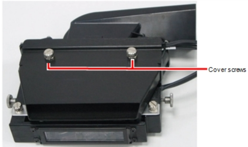
Figure 6-100 UV-lamp-cover screws
