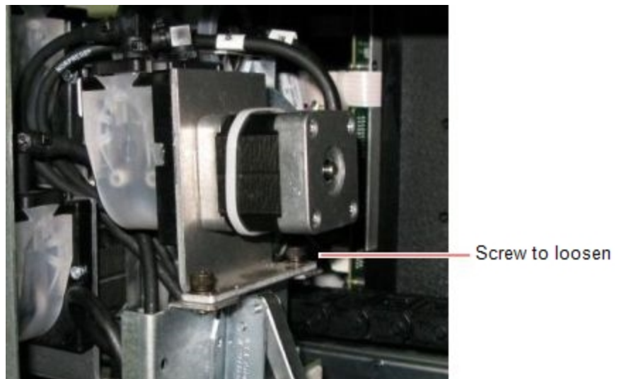
Figure 6-132 Model pump—securing screw to loosen
