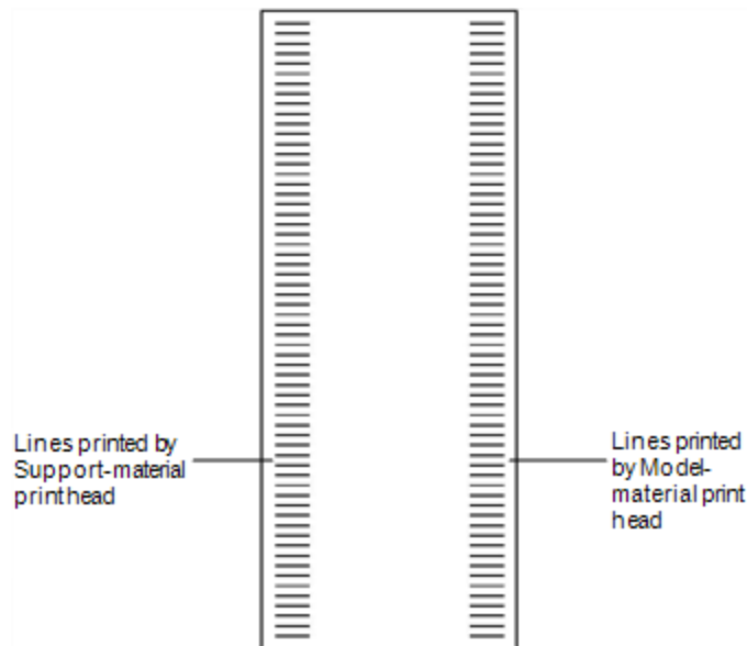
Figure 6-42 Sample Pattern Test
