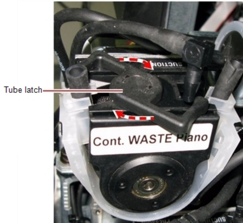
Figure 6-128 Releasing the tube latch
