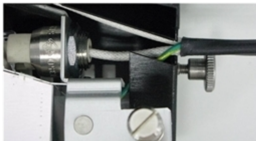
Figure 6-103 Cable position when installing the UV lamp
