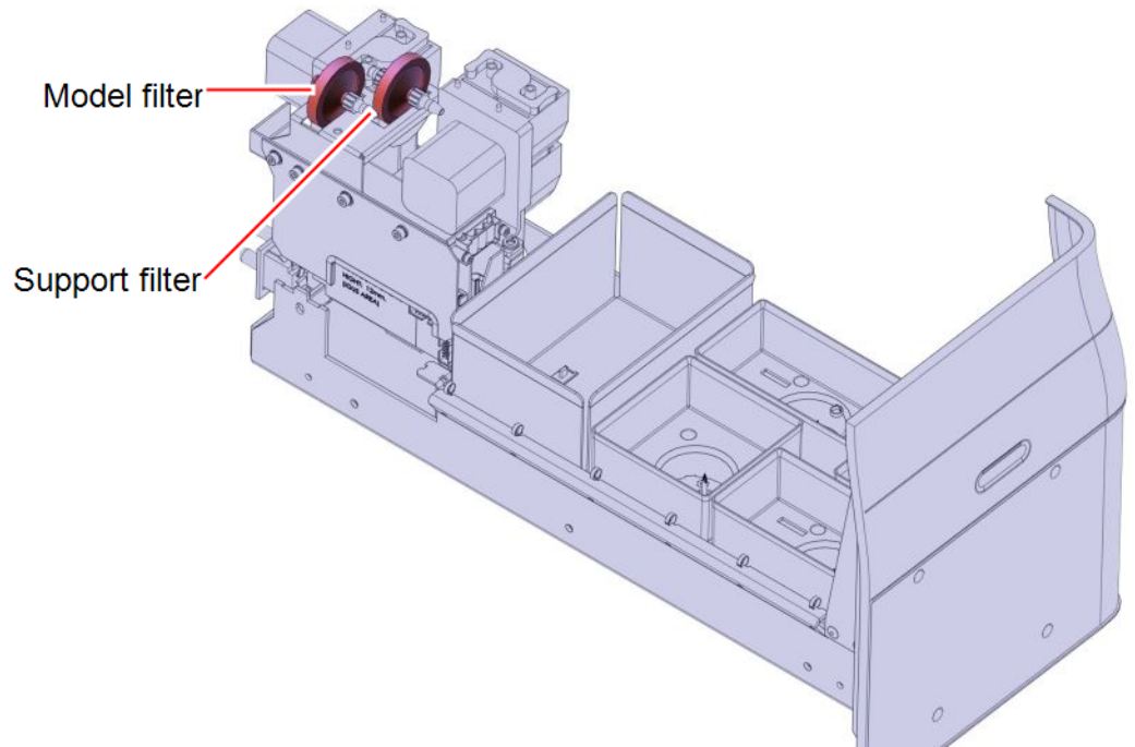
Figure 6-107 Material filters
