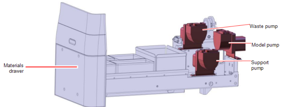
Figure 6-121 Material pumps
