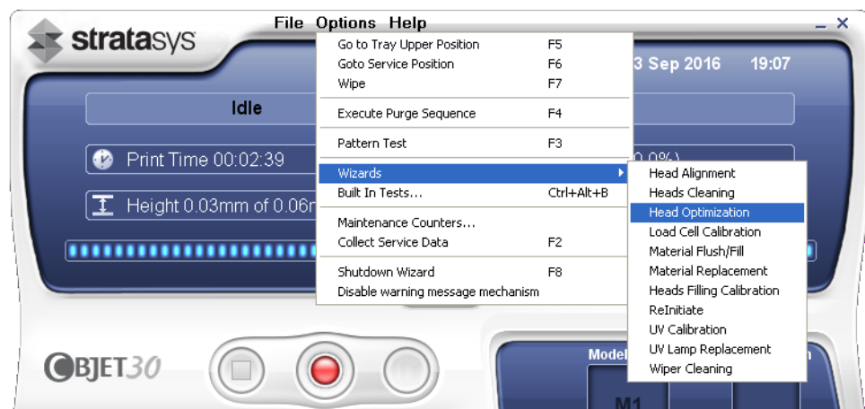
Figure 6-58 Starting the Head Optimization wizard
