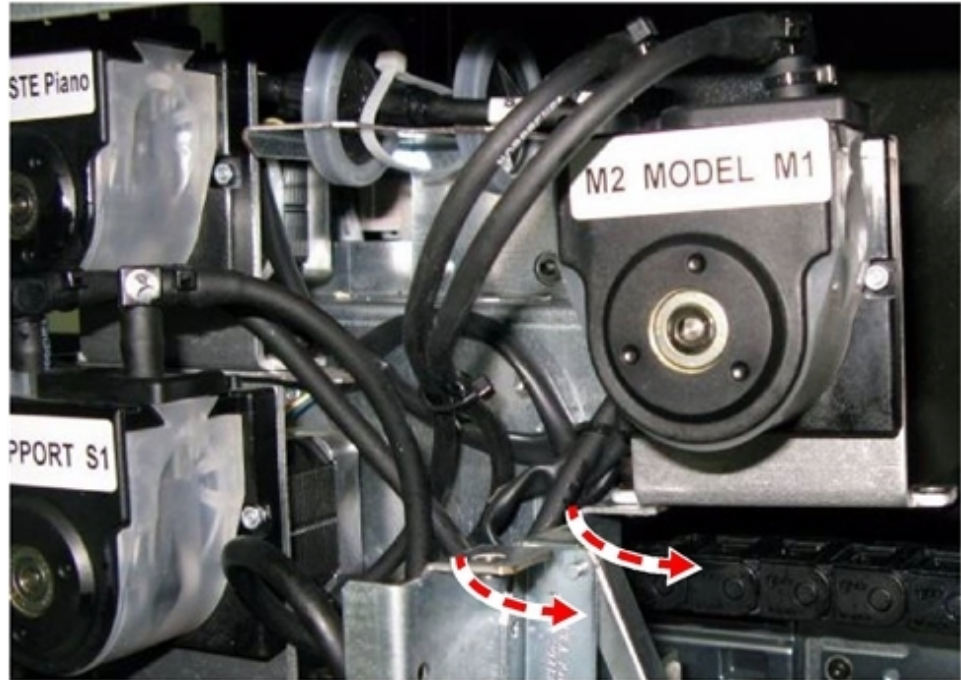
Figure 6-133 Model pump assembly turned
