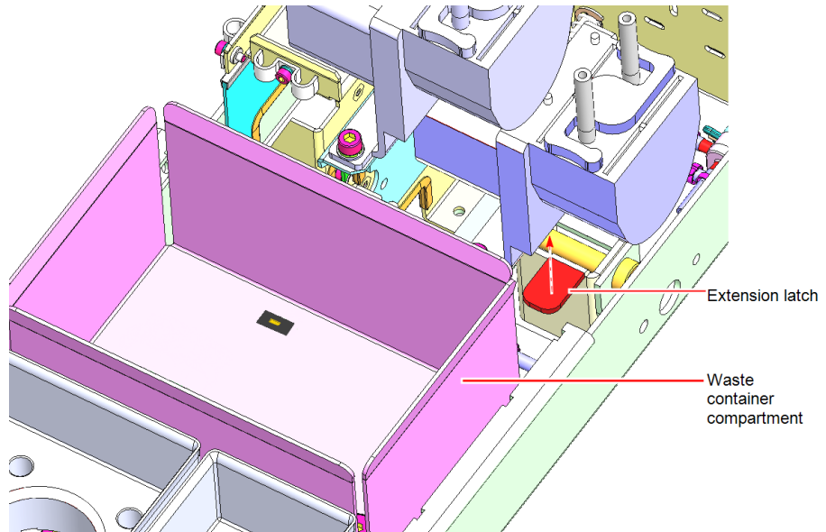
Figure 6-109 Materials drawer extension latch
