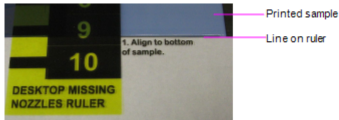
Figure 6-67 Aligning the ruler to the bottom of the sample
