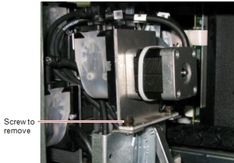
Figure 6-131 Model pump—securing screw to remove
