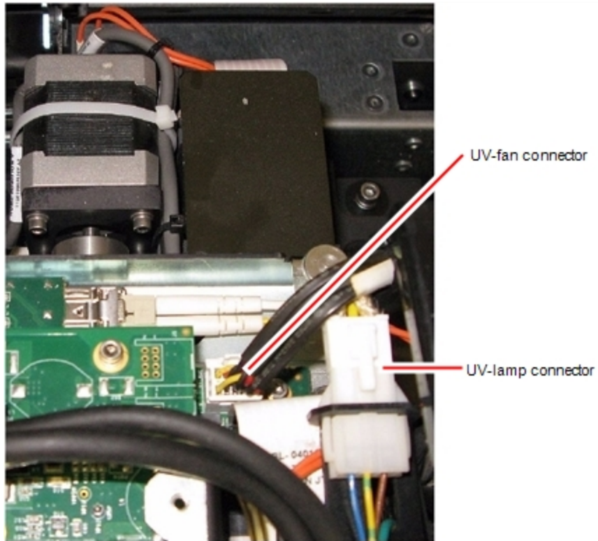
Figure 6-98 Disconnecting the UV lamp assembly (top view)
