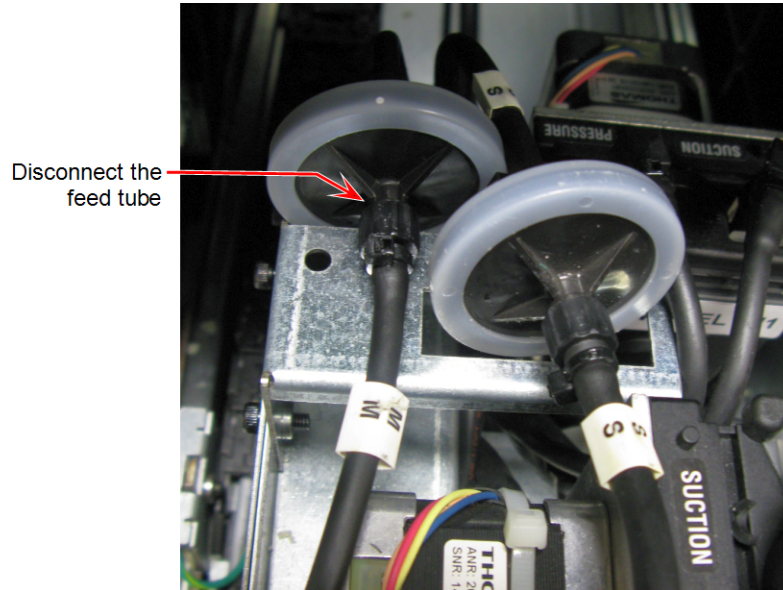
Figure 6-111 Model and Support material filters
