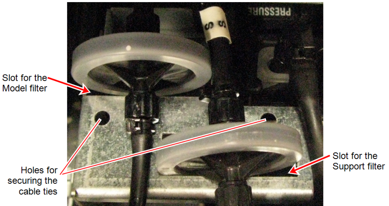
Figure 6-117 Material filters positioned in the printer
