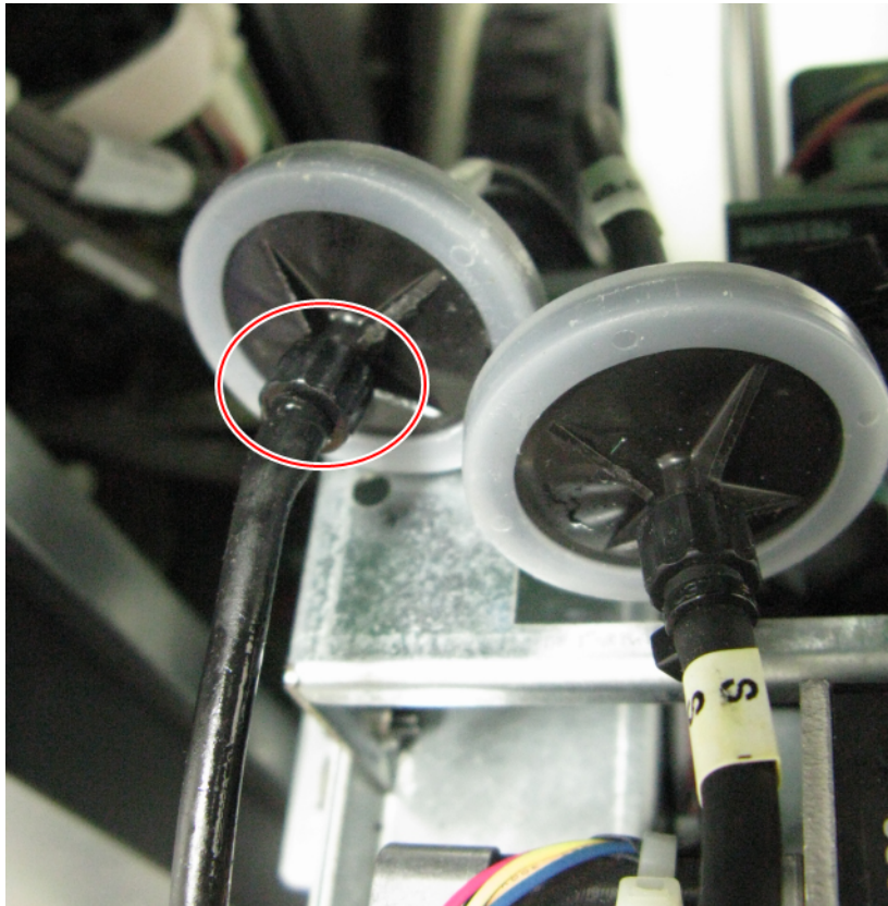
Figure 6-115 Tube attached to the new filter
