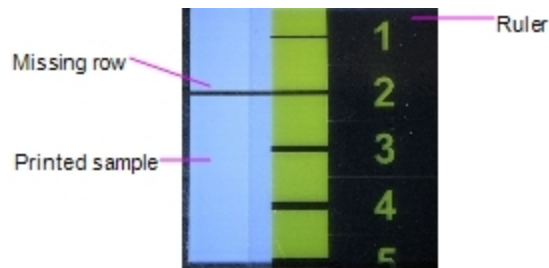
Figure 6-69 Measuring a missing row in a printed sample In the example above, the number of missing nozzles is two (2).
