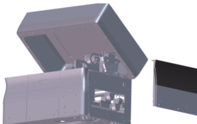
Figure 6-122 Removing the right printer panel
