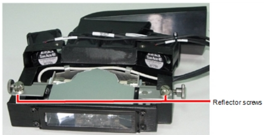
Figure 6-101 UV-reflector screws
