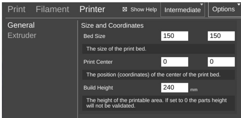
Fig. 22-17: Printer configuration.
