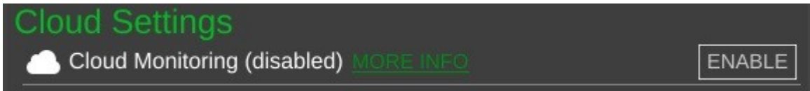
Fig. 24-7: Cloud Settings.
