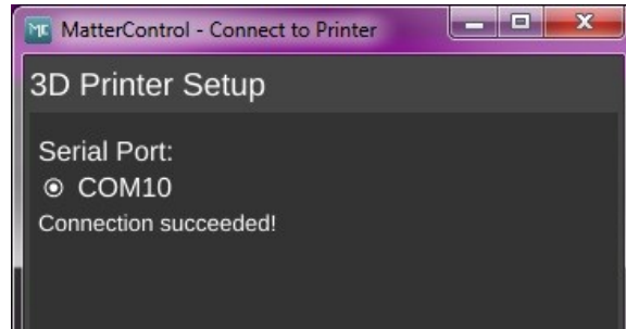
Fig. 19-8: Success!
