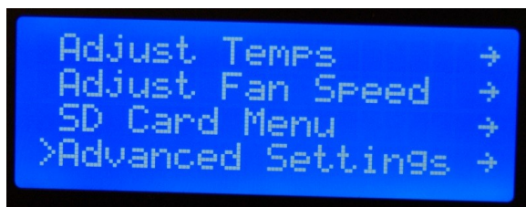
Fig. 19-25:Advanced Settings.
