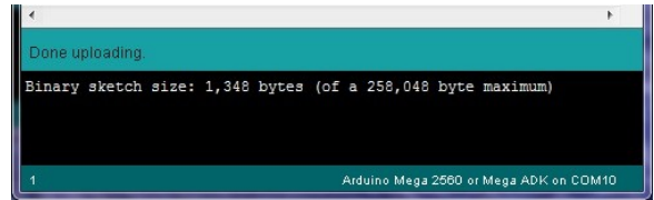
Fig. 18-6:Success!
