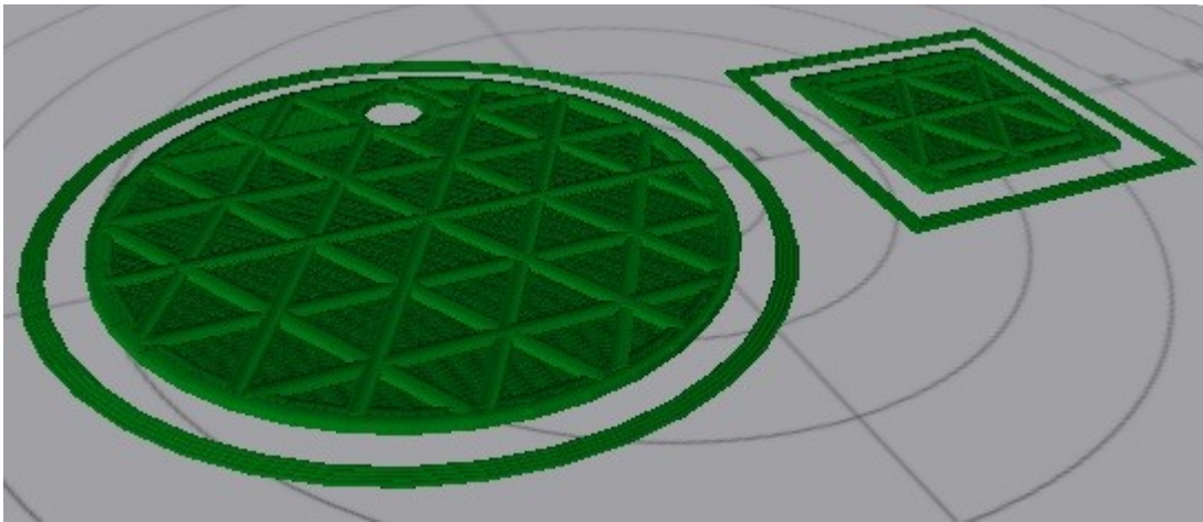
Fig. 28-6: 7 Layers in, 3D view.
