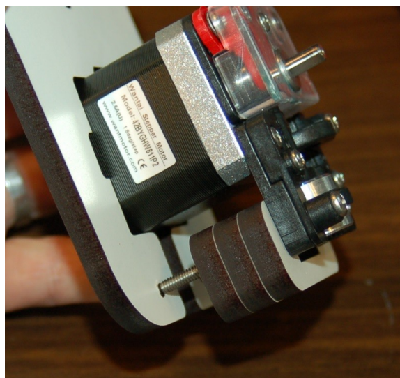
Fig. 10-14: Fitting the EZStruder to the bracket.
