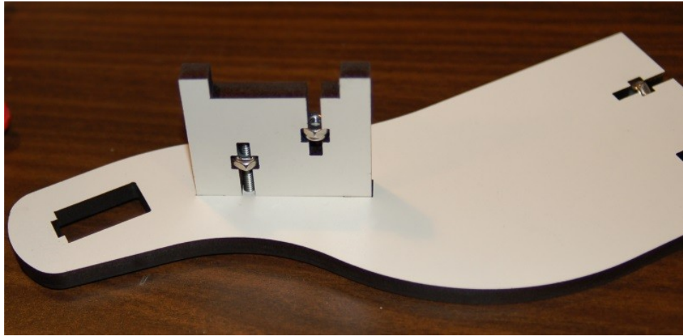
Fig. 14-2: Brace installed in inner spool support.
