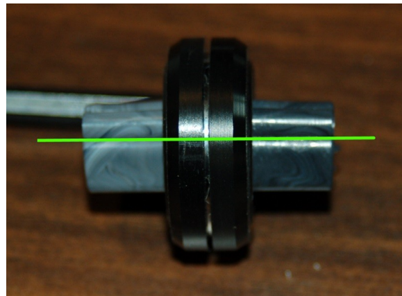
Fig. 8-18: Eccentric spacers.
