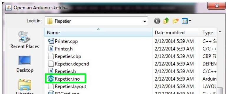
Fig. 18-7: Opening Repetier.ino
