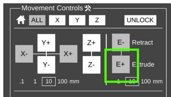
Fig. 20-15: Extruder control.
