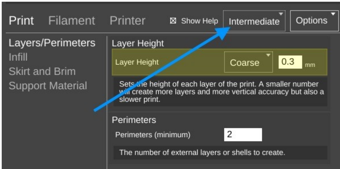
Fig. 22-9: Intermediate Settings.
