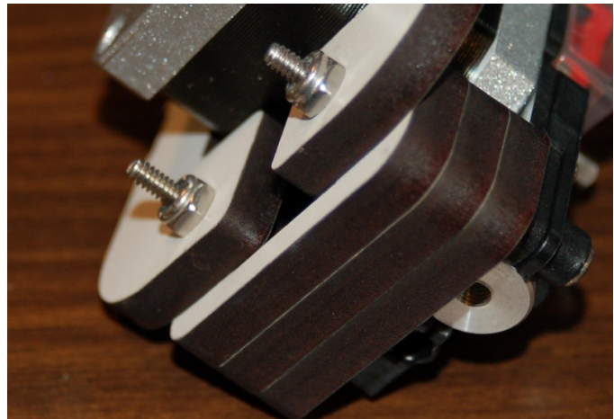
Fig. 10-15: EZStruder installed.
