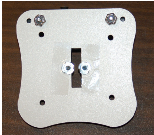
Fig. 8-16: T-Nuts installed.
