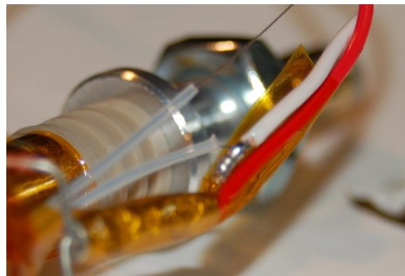
Fig. 11-19: Thermistor lead soldered to white wire.
