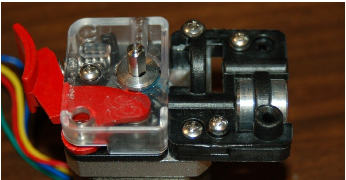
Fig. 10-9: Assembled EZStruder.
