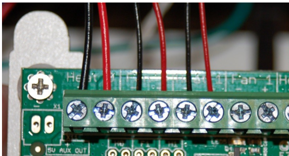
Fig. 16-28: PEEK fan wires installed.
