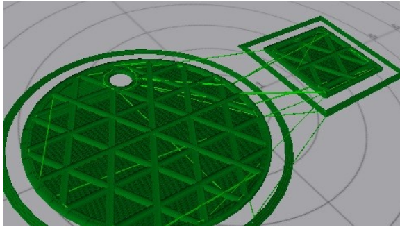
Fig. 28-7: Travel moves.
