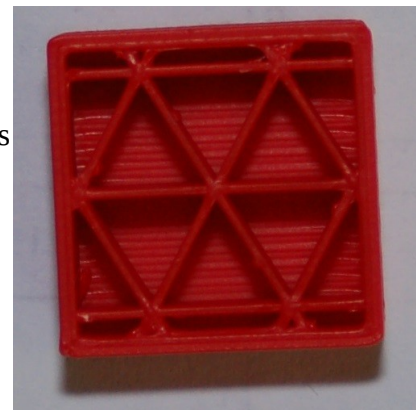
Fig. 22-4: 20% infill example.
