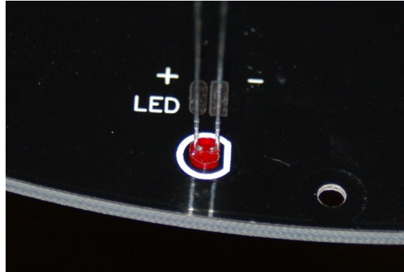
Fig. 5-9: LED orientation.
