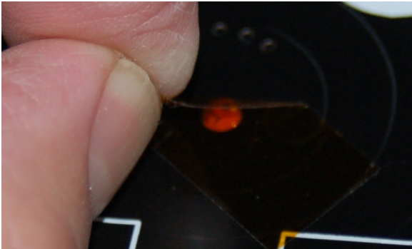
Fig. 17-16: Kapton removal.
