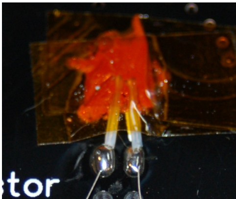
Fig. 5-7: Soldered down..
