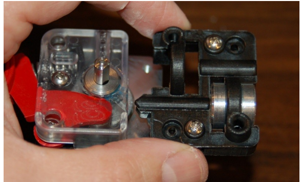
Fig. 10-7: Filament guide block orientation.
