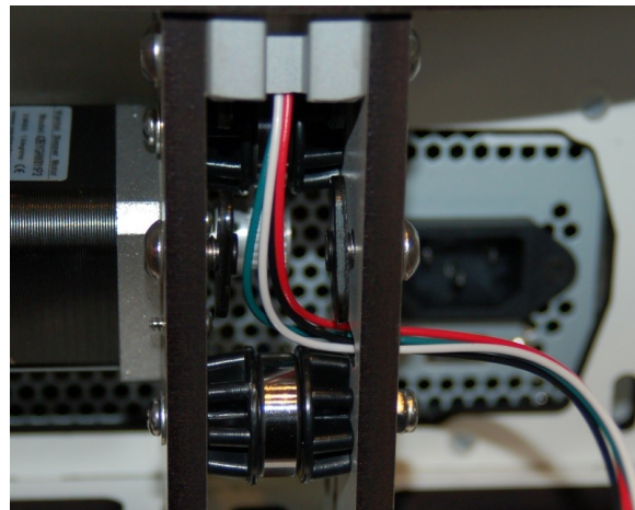
Fig. 6-16: Wire route.
