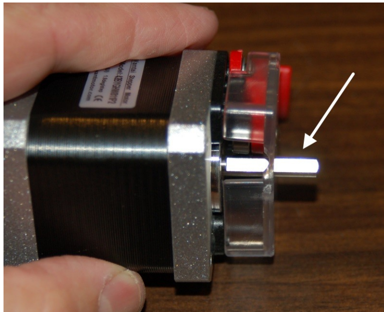
Fig. 10-4: Shaft aligned.
