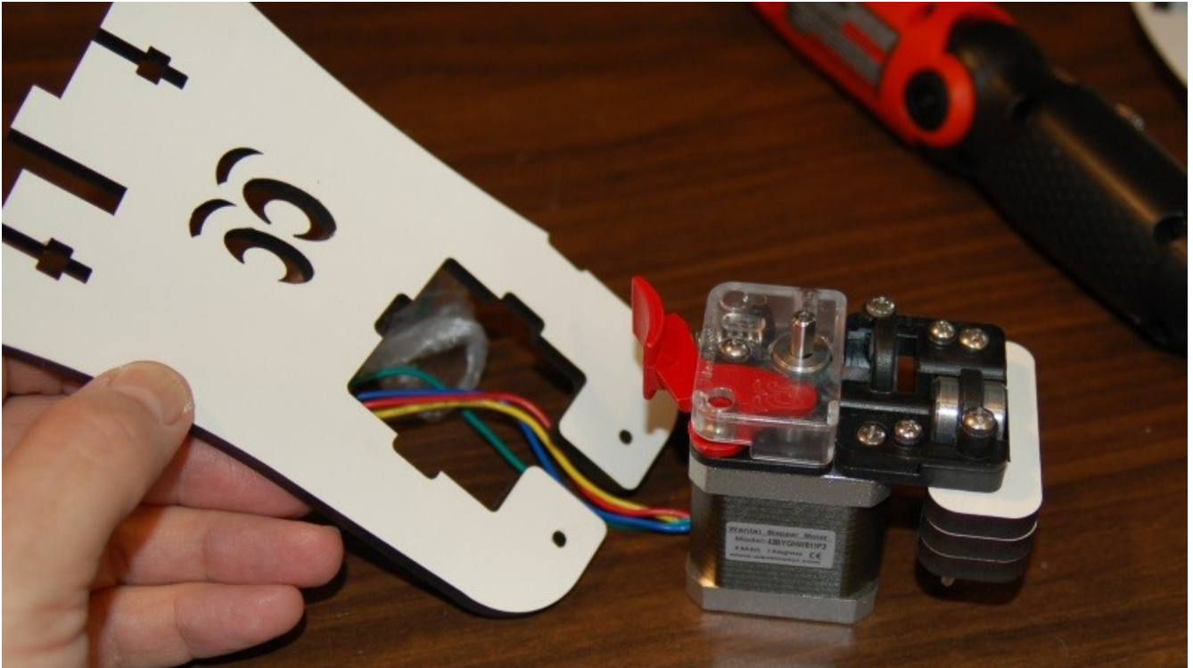
Fig. 10-13: Bracket & EZStruder orientation.
