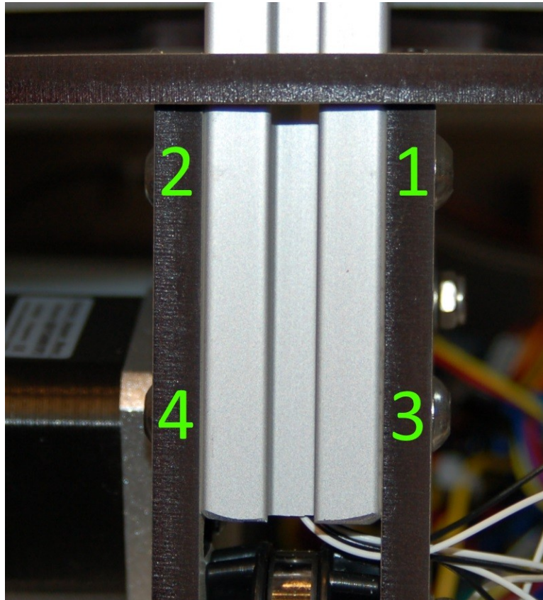
Fig. 7-51: Tightening order.
