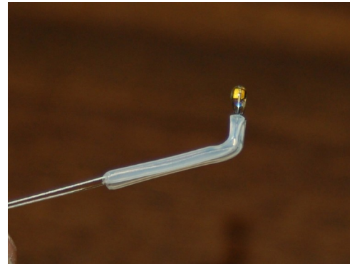
Fig. 5-3: 90 degree bend.
