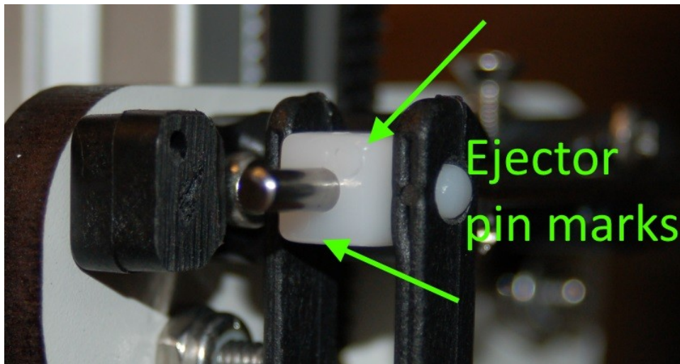
Fig. 12-10: Installing a delta arm.
