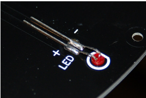
Fig. 5-11: Leads soldered into place.
