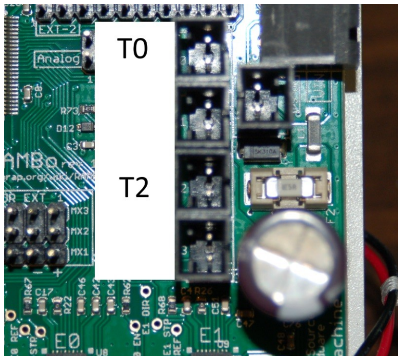
Fig. 16-32: Thermistor connectors.
