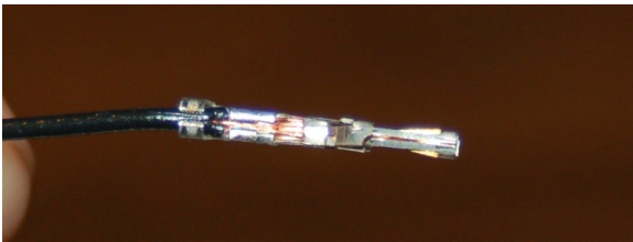
Fig. 16-24: First of four crimps.
