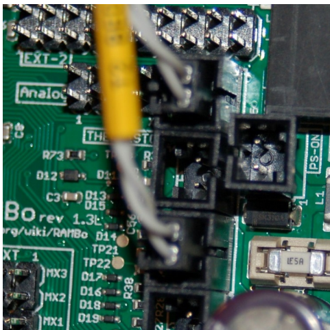
Fig. 16-33: Thermistors plugged in.
