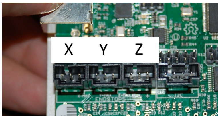
Fig. 16-30: End stop connector plugs.
