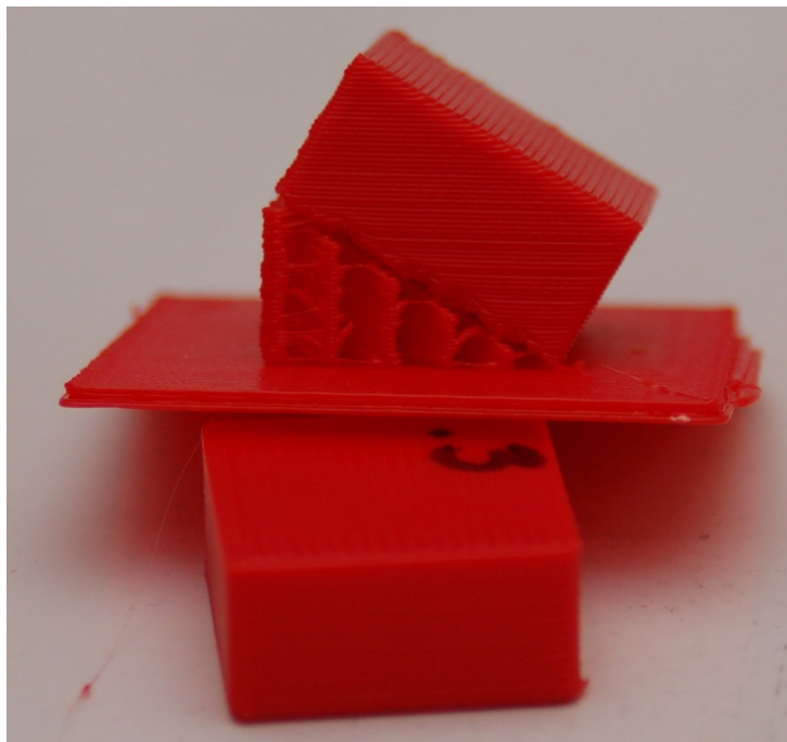
Fig. 22-6: Support & Raft.
