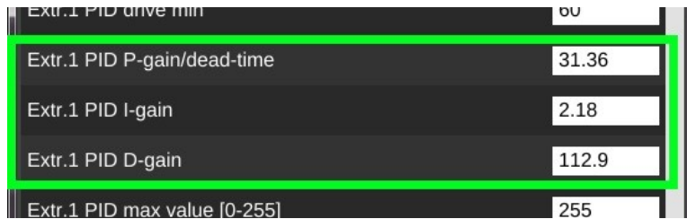
Fig. 19-24: Extruder PID settings.
