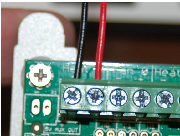
Fig. 16-26: Hot end wires installed.
