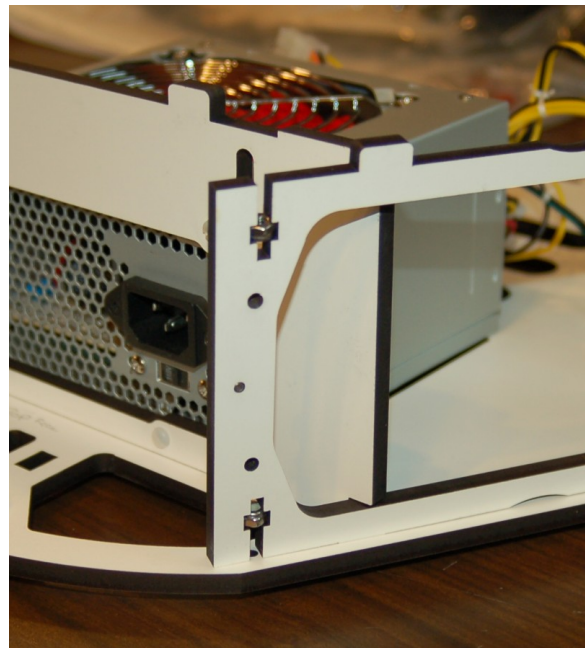
Fig. 4-20: Right side fully seated.
