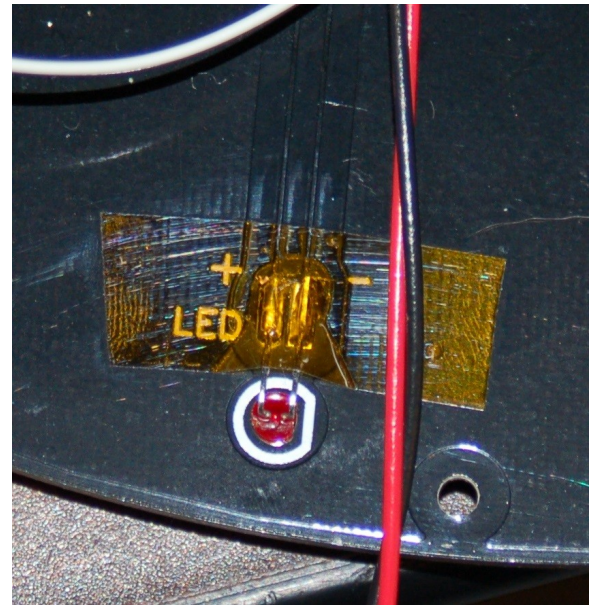
Fig. 5-26: LED covered.
