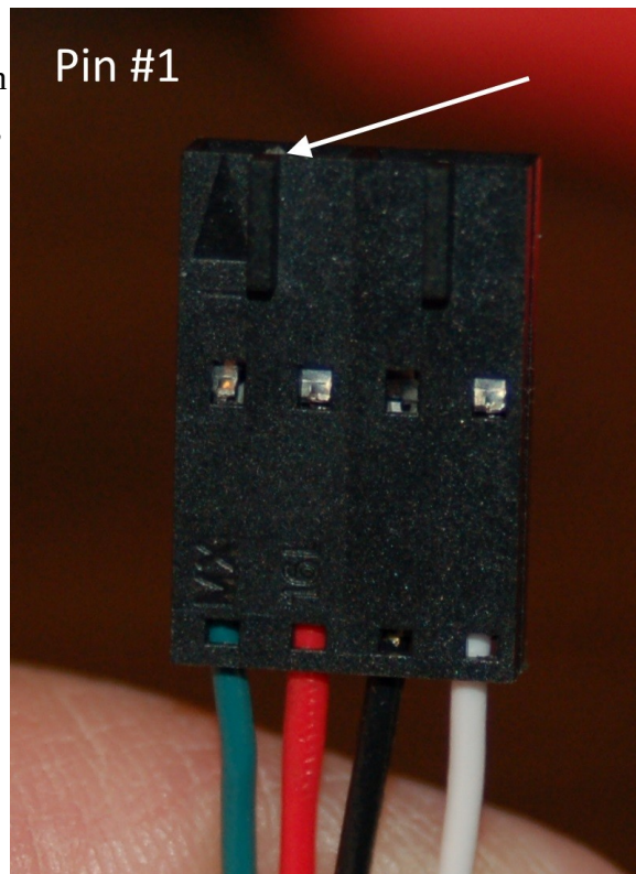
Fig. 16-25: Connector wire order.
