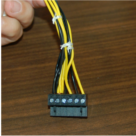
Fig. 3-29: Bundled up!
