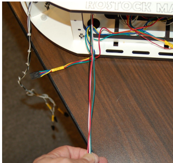
Fig. 16-18: Working length for hot end & thermistor wires.
