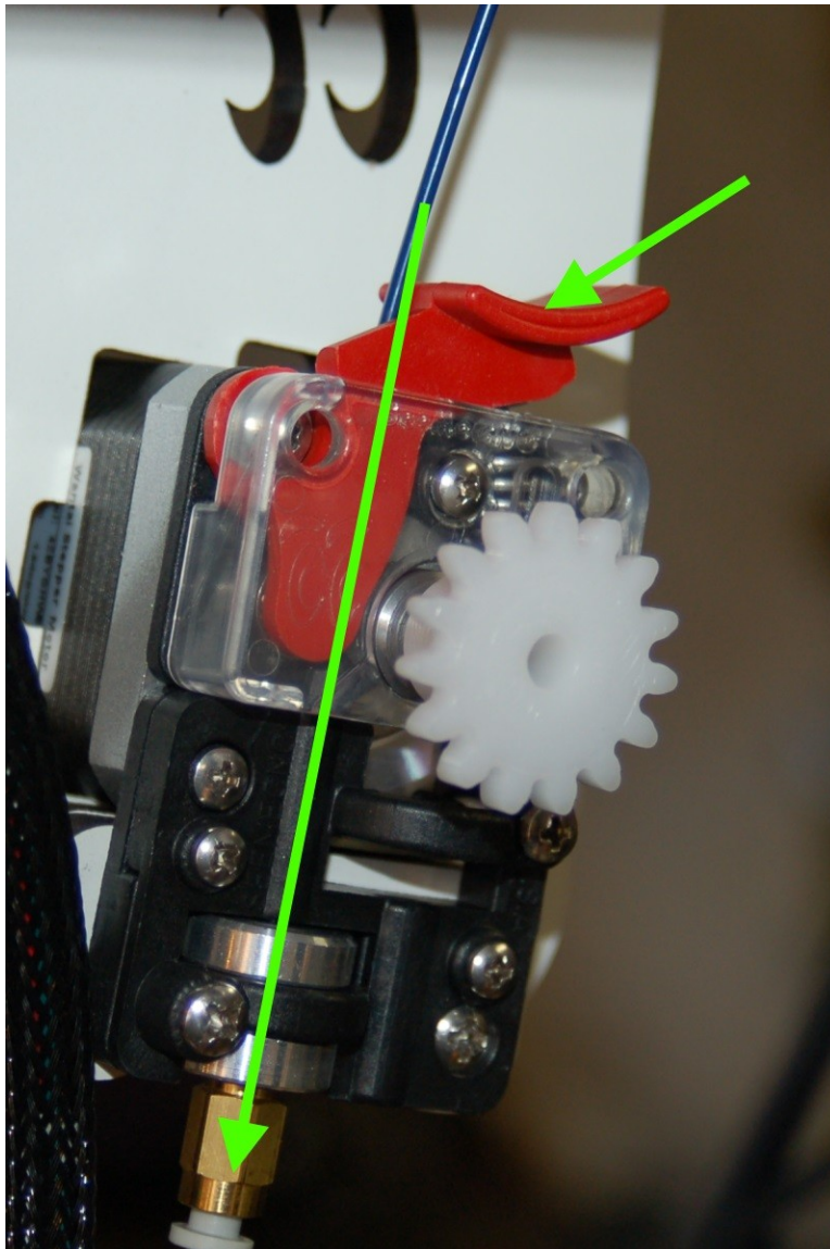
Fig. 20-14: Loading filament.
