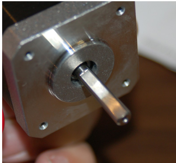
Fig. 4-26: Flatted shaft.
