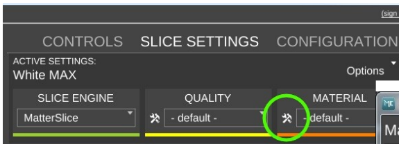
Fig. 20-5: Materials Toolbox.
