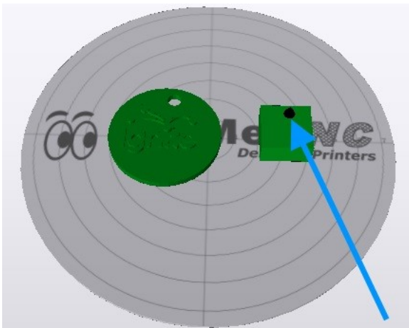
Fig. 28-2: Object selected.
