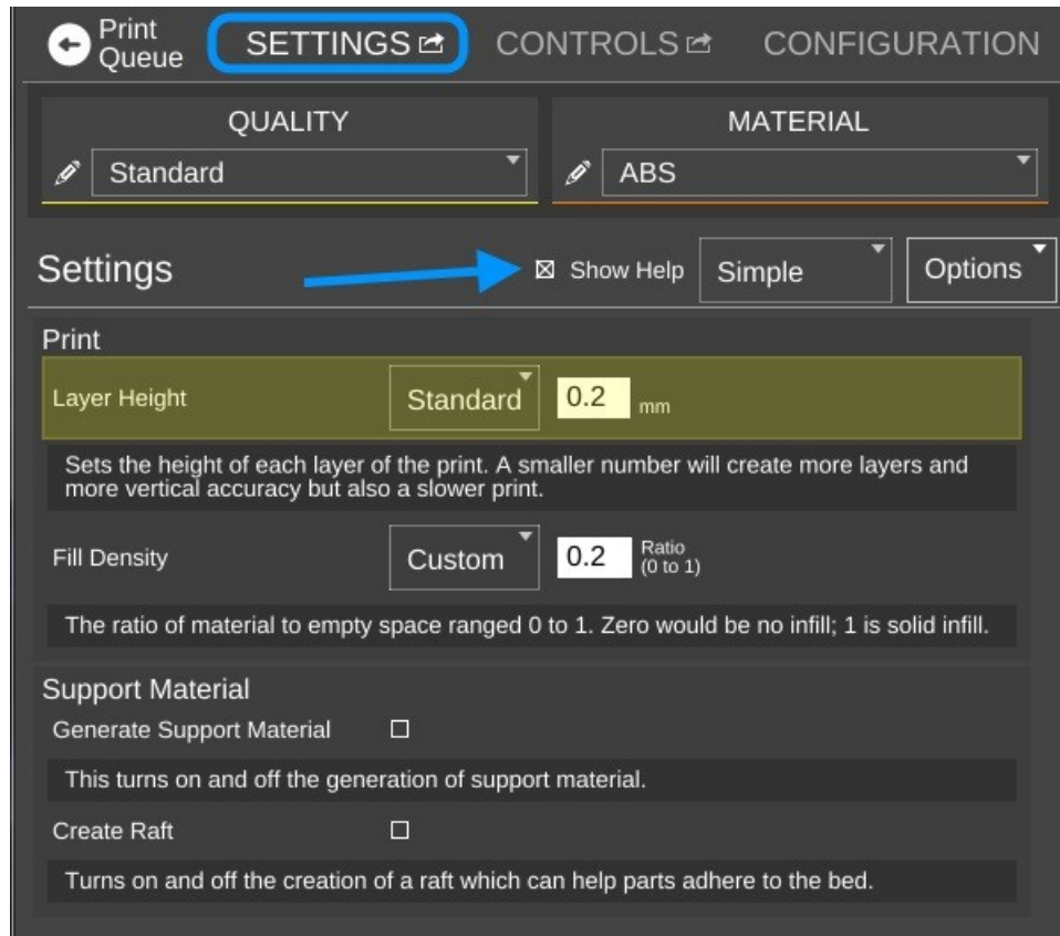
Fig. 22-2: Settings Pane.
