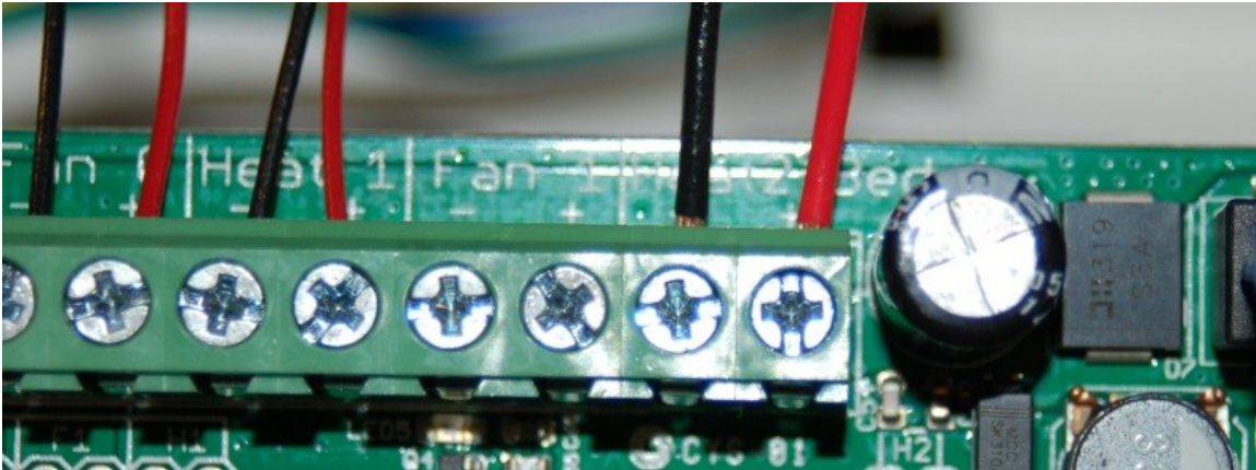
Fig. 16-29: Heated bed wires installed.
