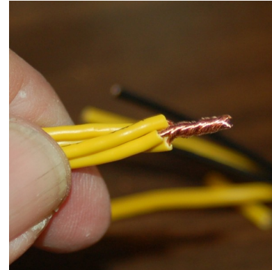
Fig. 3-25: Primaries bundled.
